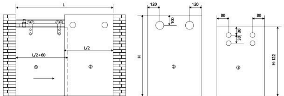
Φ25 管浴室吊轮平面安装图 Installation of Φ25 pipe bathroom hanging wheel
