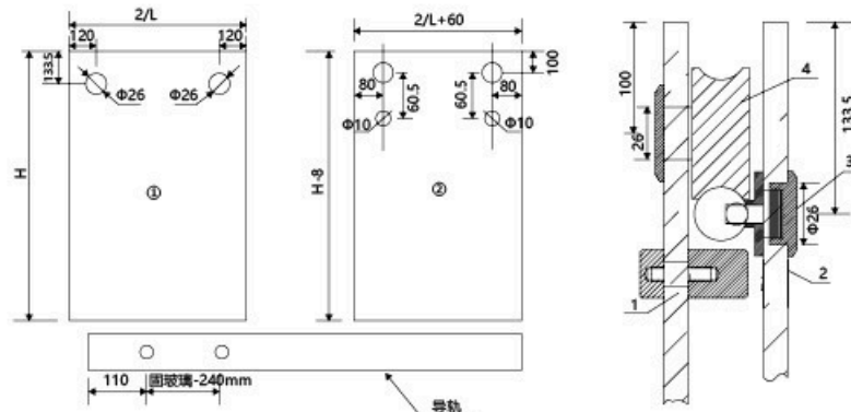
Φ25 管浴室吊轮截面安装图 Sectional Installation of Φ25 Pipe Bathroom Hanging Wheel
