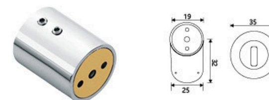
AT-E005 圓形靠牆管套 Round wall sleeve
