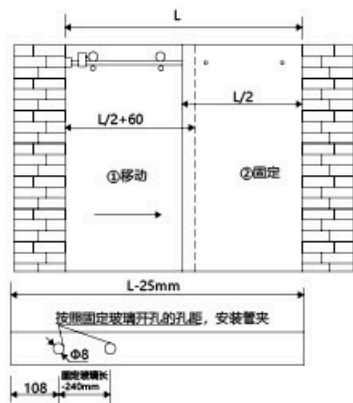
30X10 方管帶防跳平面安裝圖 30X10 installation of square pipe with jumping-proof pillar
