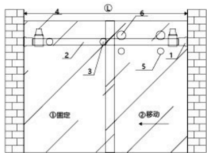
Φ25 管浴室吊轮平面安装图 Installation of Φ25 pipe bathroom hanging wheel
