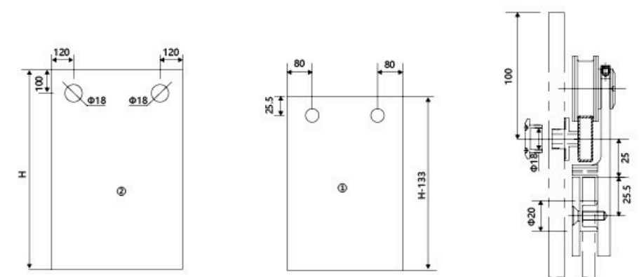
30X10 方管截面安装图 Sectional Installtion Map with 30*10 Square Pipe
