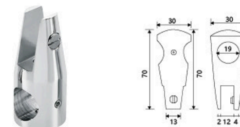
AT-E003 圓形圓錐吊夾 Circular conical hanging clamp
