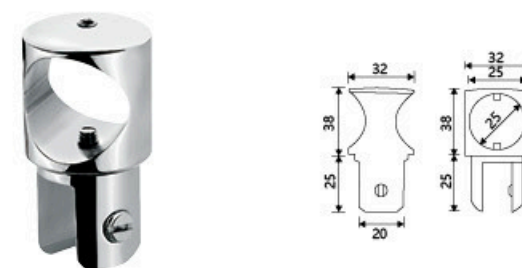
AT-E002 圓形吊夾 Round hanger
